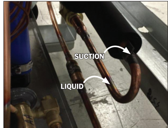
Fig. 5 Refrigeration suction and liquid connections
