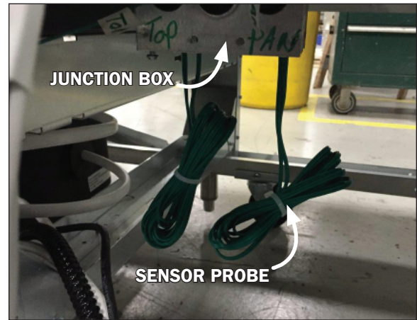
Fig. 9 Field-wired sensors
